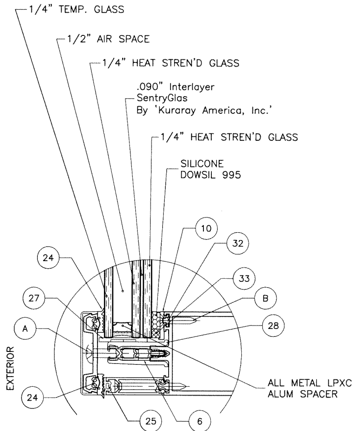
GLASS TYPE 'Ai' 1-5/16" OVERALL NOMINAL THK.
