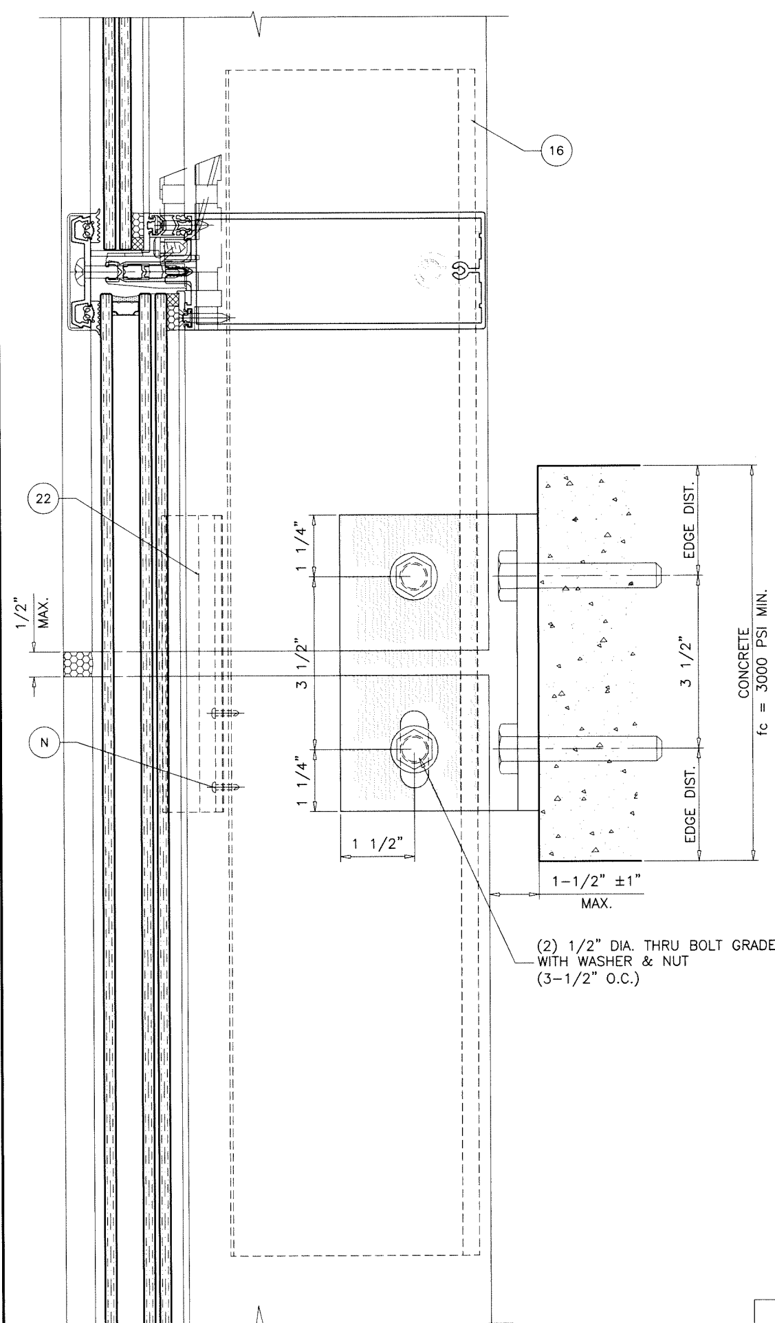
INTERMEDIATE ANCHORS
