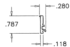
10 SSG GLAZING ADAPTER
