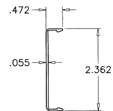
5 FACE COVER (HORIZONTAL)
