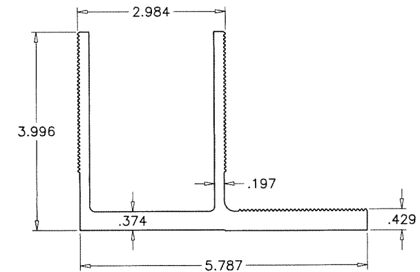
20 'F' CLIP (INTERMEDIATE)
