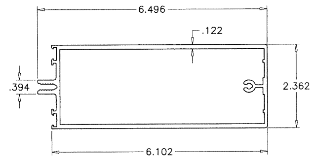
2 FRAME HEAD/SILL/HORIZONTAL
