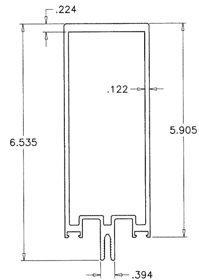
1 JAMB/MULLION
