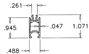
8 GLAZING ADAPTER
