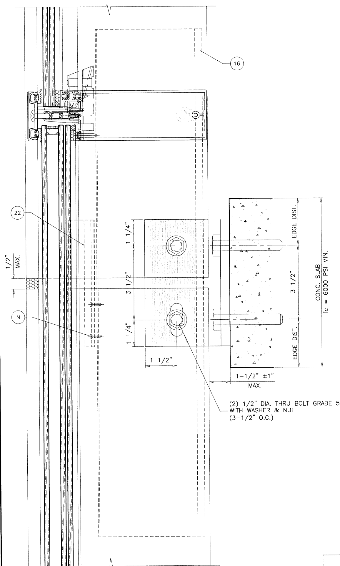
INTERMEDIATE ANCHORS
