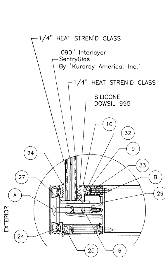
GLASS TYPE 'A' 9/16" OVERALL NOMINAL THK.
