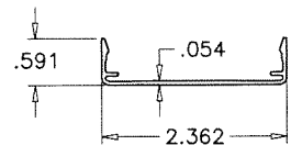
4 FACE COVER (VERTICAL)
