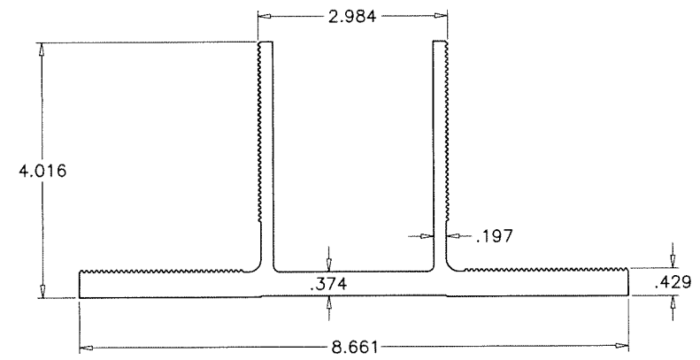
21 'T' CLIP (INTERMEDIATE)
