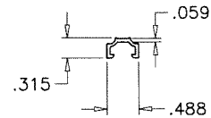
7 GLAZING ADAPTER
