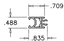
9 GLAZING ADAPTER
